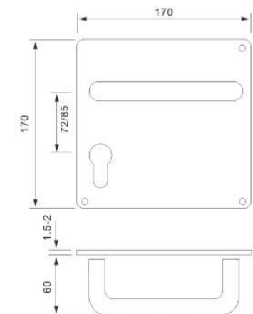
HP.SB100C.SS Material: Stainless Steel Finishing: SS/PSS/DAB/PVD
